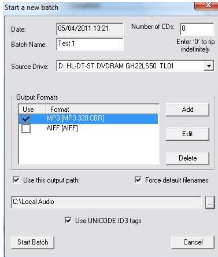
Figure 4.8 – Start a New Batch Dialog Box
